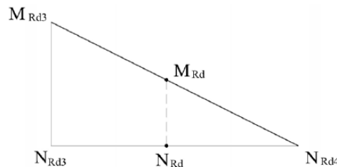
Figure 6.8. Terminal end of the interaction diagram M-N
