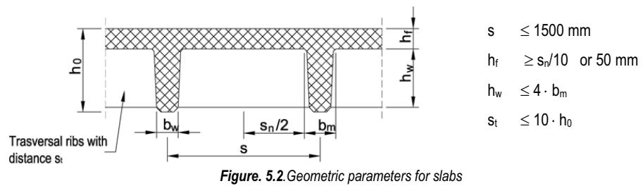
Figure 5.2. Geometric parameters for slabs
