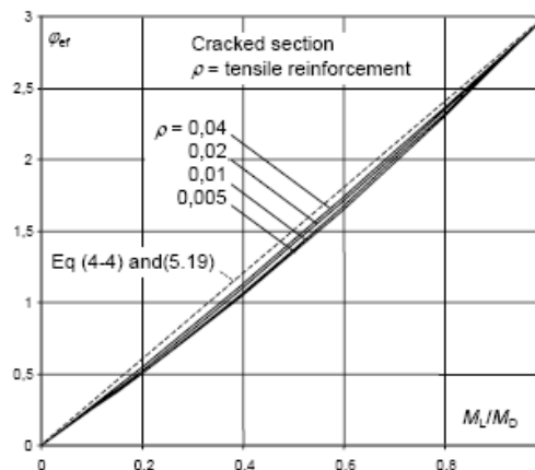
Figure 5.22. Effective creep ratio as a function of ratio M_t/M_0 for a cracked rectangular cross section with tensile reinforcement only, based on d = 0.9h and \alpha = 6 . Basic creep coefficient \phi = 3
