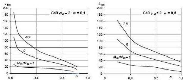
Figure 5.11. Effect of reinforcement ratio on slenderness limit (only criterion 1 is shown here).
