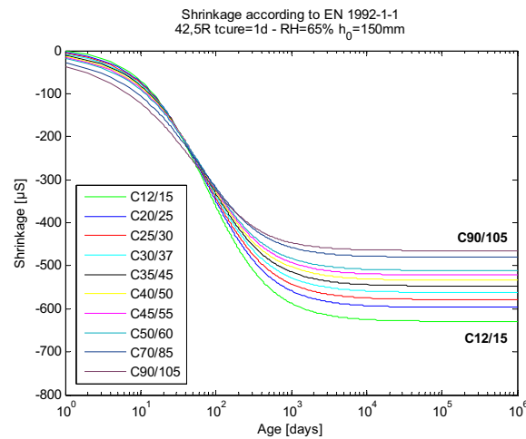
Figure 3.2. Development of shrinkage according to EC2
