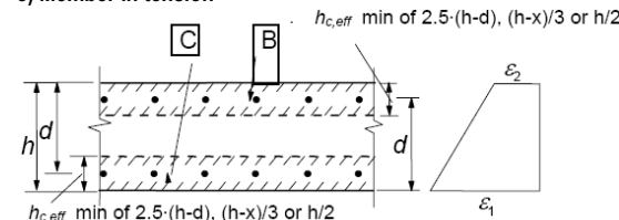
Figure 7.9 Definition of the effective tension area
